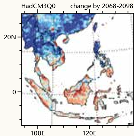
Figure 6. Projected changes in mean annual maximums of extreme rainfall events from HadCM3Q0 for mid-century (top) and end-century (bottom). Red shades show decreasing rainfall intensities (mm/day), blue shades show increasing rainfall intensities.
