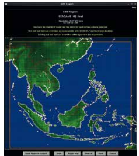
Figure 3. Domain used in the model experiments. This area encompasses each of the ASEAN member countries.
