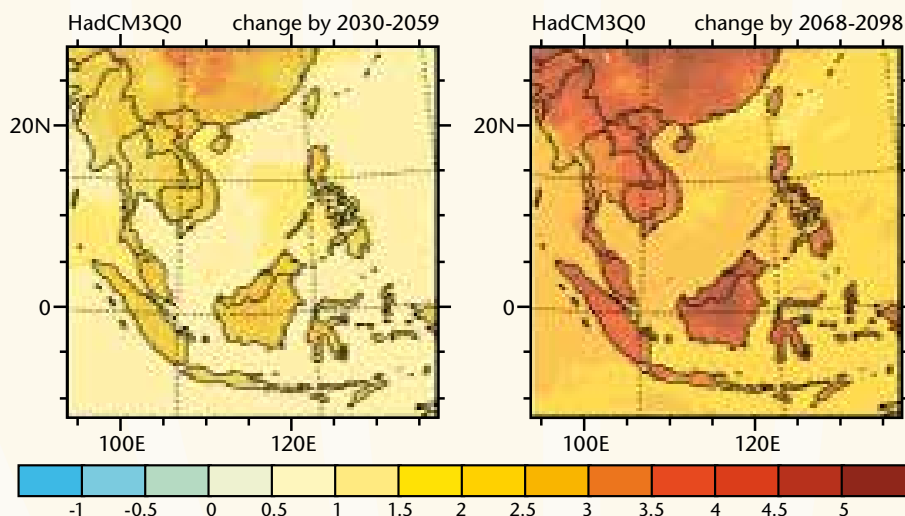
Figure 5. Projected changes in annual mean temperature (annual maximum daytime temperature in °C) from HadCM3Q0 for mid-century (left) and end-century (right). Darker red shades show stronger areas of temperature increase compared to the baseline temperatures; 1970-2000.
