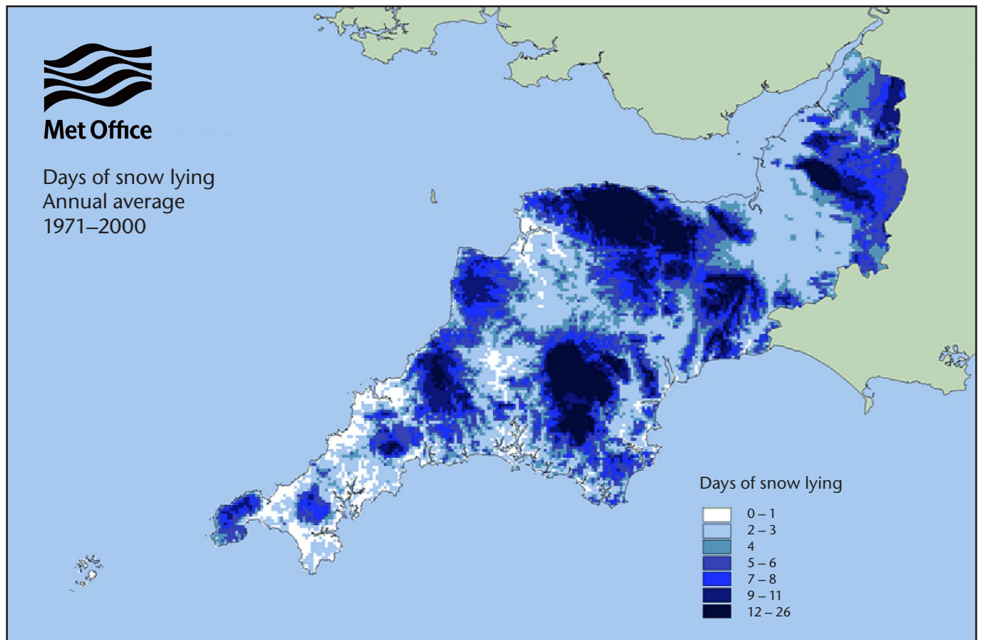
Figure 19. Map showing the 30-year (1971–2000) average number of days per year with snow lying.
