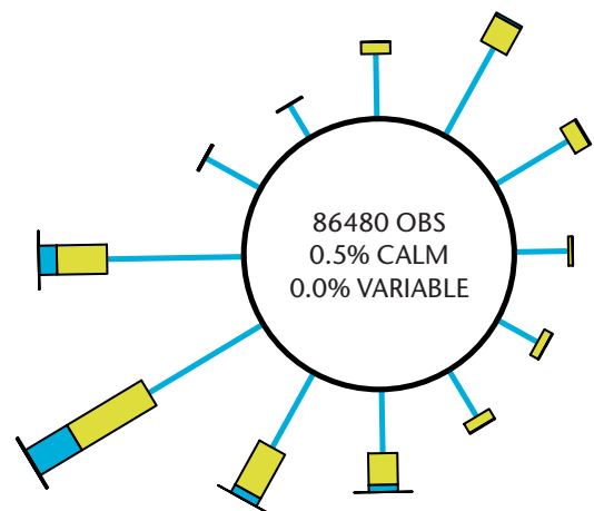
Wind rose for the period 2004–2013 at Exeter (27 metres above mean sea level)
