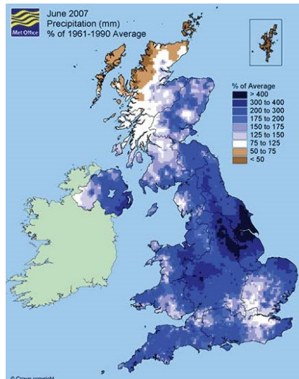
Left Map showing percentage of average June rainfall over the U in June 200 showing over 00 across much of or shire an Hum ersi e Right rainfall totals an percentage of 19 1 1990 average for the U an then y area
