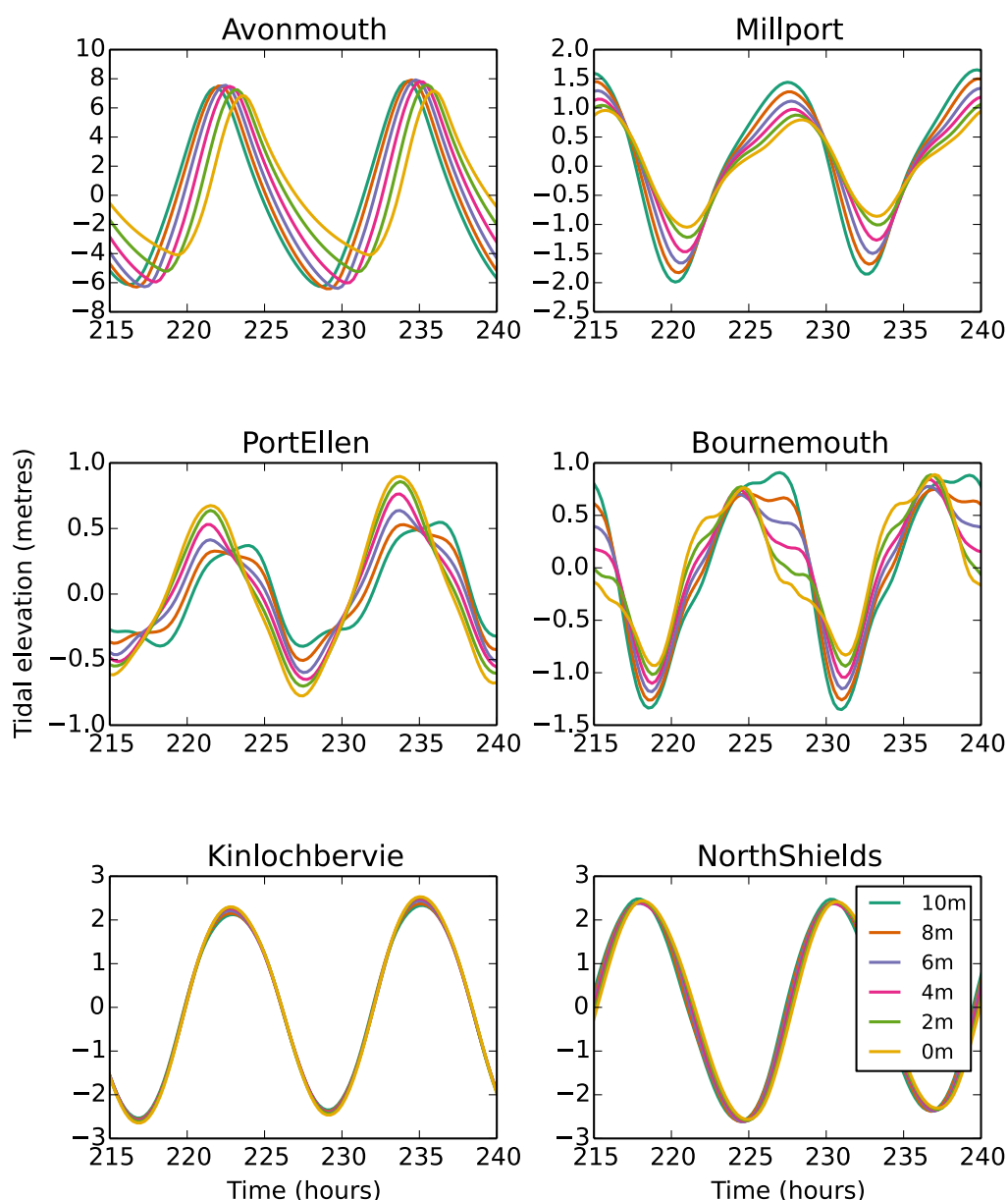
Figure 4.3.1. Example modelled changing tidal cycles at six selected locations under time-mean sea level increases of up to 10 metres, in steps of 2 metres. The legend shows the imposed time-mean sea level increase. Time is shown in hours since the 'cold' start (i.e the start of the spin-up from flat sea surface). We vary the Y-axis of these plots to accommodate the large spatial variability in the tidal range. The direct effect of the imposed time-mean sea level change is not shown: what is shown here is the tide relative to the imposed time-mean sea level. More long-term (potential millennial-scale, c/f section 3.1.2) time-mean sea level increases up to 10 metres are included as a test of the proportionality of the response. There is no implication that such high levels will be realised within the next two centuries.
