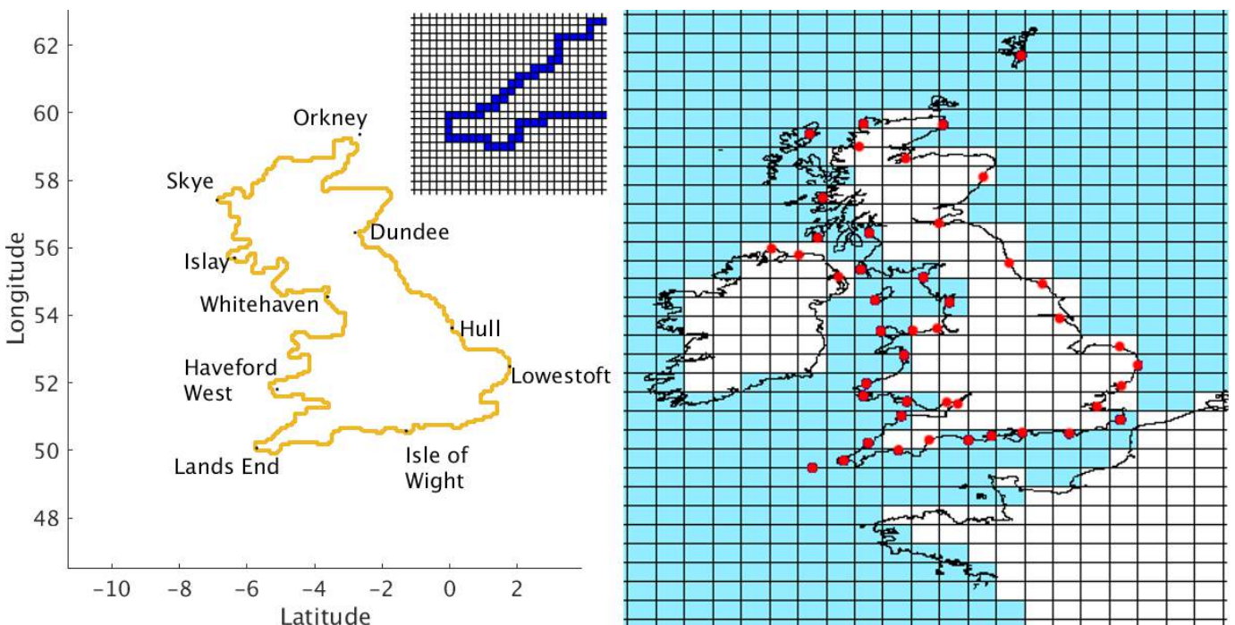
Figure A1.6.2. Regional wave model grid points where coastal strip plots are extracted from (left), and locations of class-A gauges used, with corresponding global wave model grid (right). An inset showing the regional model resolution around SW England is shown in the left-hand panel.
