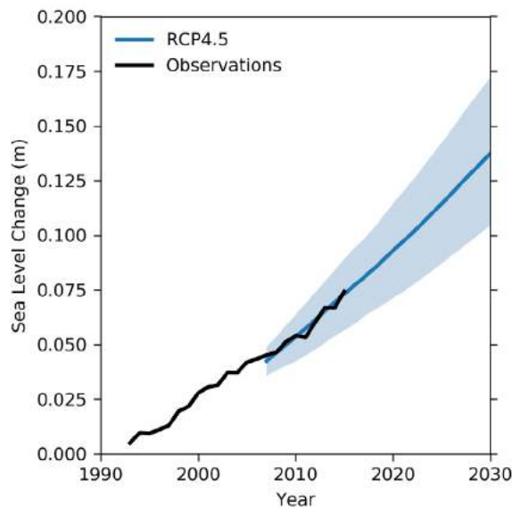
Figure 3.1.2. Comparison of the UKCP18 global time-mean sea level projection for RCP4.5 with the annual mean values from satellite altimetry observations (ESA CCI Sea Level data version 2.0; http://www.esa-sealevel-cci.org/ ). The sea level projections are shown relative to a 1981-2000 baseline period. The satellite observations are plotted so that they match the average of the projection time series for the overlapping period of 2007-2015.
