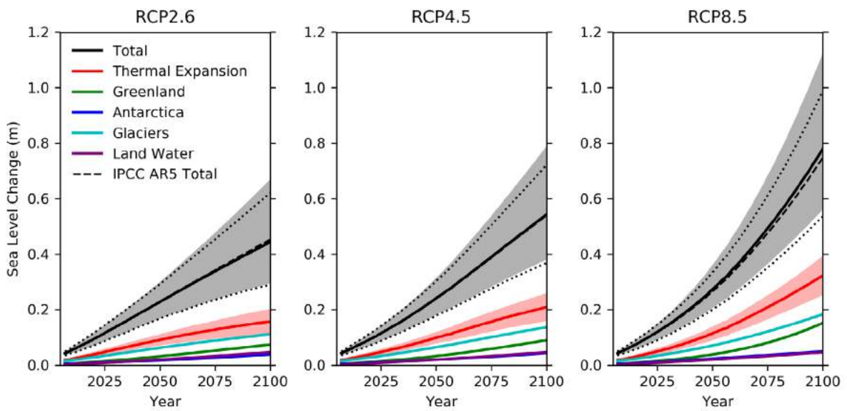
Figure 3.1.1. UKCP18 global time-mean sea level projections for the 21 st century, including components as indicated in the figure legend. The corresponding shaded regions indicate the range of projections for the total and thermal expansion. Also shown is the total for the sea level projections presented in the IPCC AR5 (Church et al, 2013), with the range indicated by the dotted lines. All projections are shown relative to a 1981-2000 baseline period.
