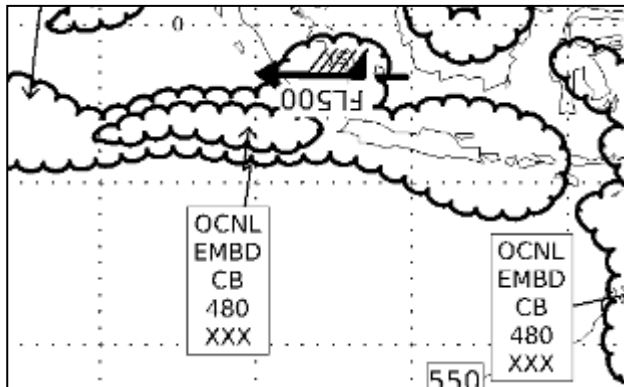
Figure 5: Easterly jetstream, just south of the equator.
