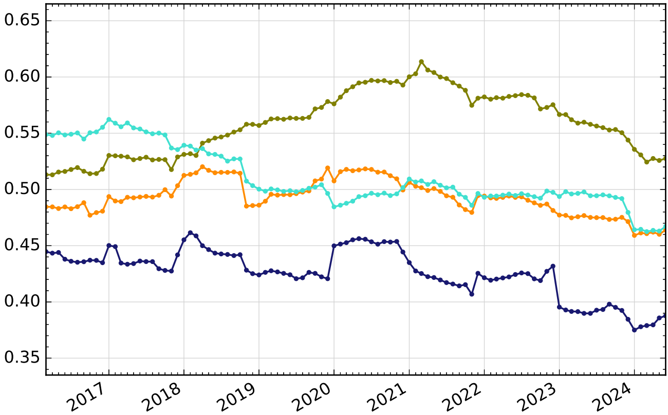
Cloud Base
